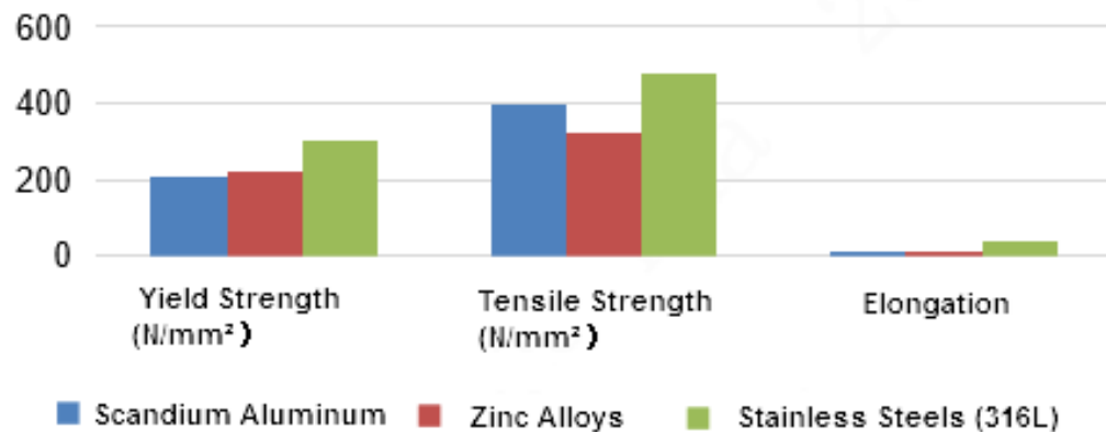
Figure 3.5 Tensile test performance parameters for different materials
